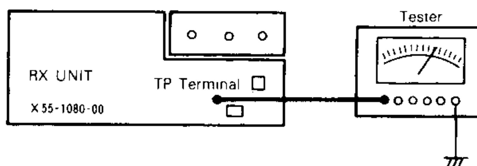
FIG. 17 NB ADJUSTMENT
